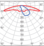
DA = Ottica stradale e ciclopeditonale estensiva Classe P - Type II/III (long) ad elevata interdistanza Extensive road and cycle-pedestrian optic Class P - Type II/III (long) for high pole spacing
