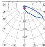
TD = Ottica centrale controflusso Central optic for counterflow
