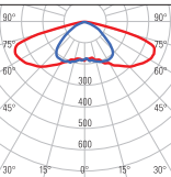
TA = Ottica tesata centro strada, permanente centrale gallerie a 2 corsie Suspended optic road center, permanent central for 2-lane tunnels
