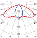
TB = Ottica tesata centro strada, permanente centrale gallerie a 1 corsia Suspended optic road center, permanent central for 1-lane tunnels
